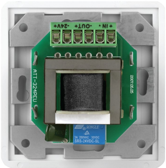
Volume Control
